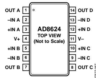
Figure 3. 14-Lead TSSOP
